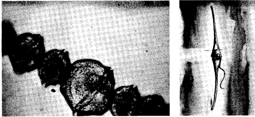
Figure 8.1 Gonyaulax ( Protogonyaulax ) catenella (above left), the chain-forming dinoflagellate responsible for paralytic shellfish poisoning in Puget Sound. The enlarged cell (center) has been infected by the parasitic dinoflagellate Amoeboophyra ceratii , and will soon burst and die. Actual size approximately 30 micrometers per cell. (Photo courtesy Louisa Nishitani). Ceratium fusus (above right), a spiny dinoflagellate linked to oyster larvae mortality in the southern Sound. Actual length approximately 100 micrometers. (After Cardwell et al., 1977)
